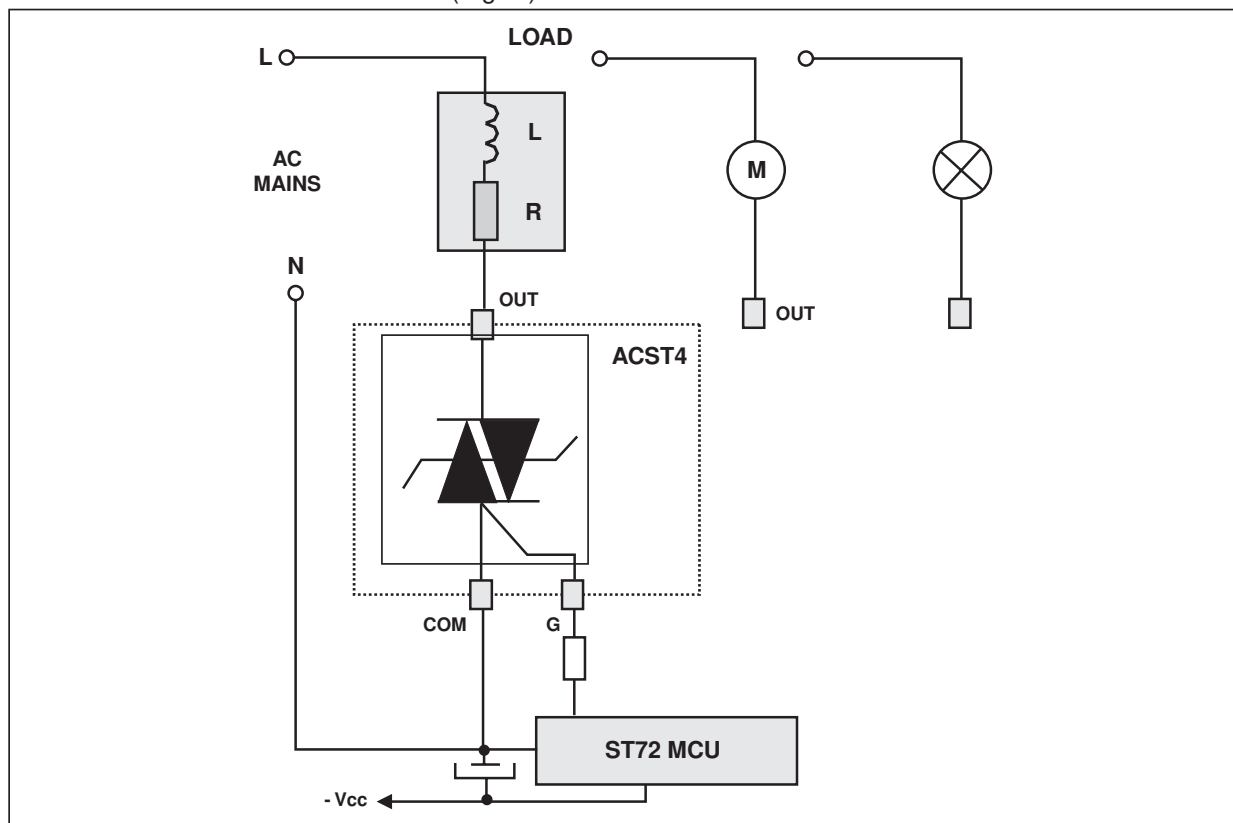
TYPICAL APPLICATION DIAGRAM (Fig. A)
