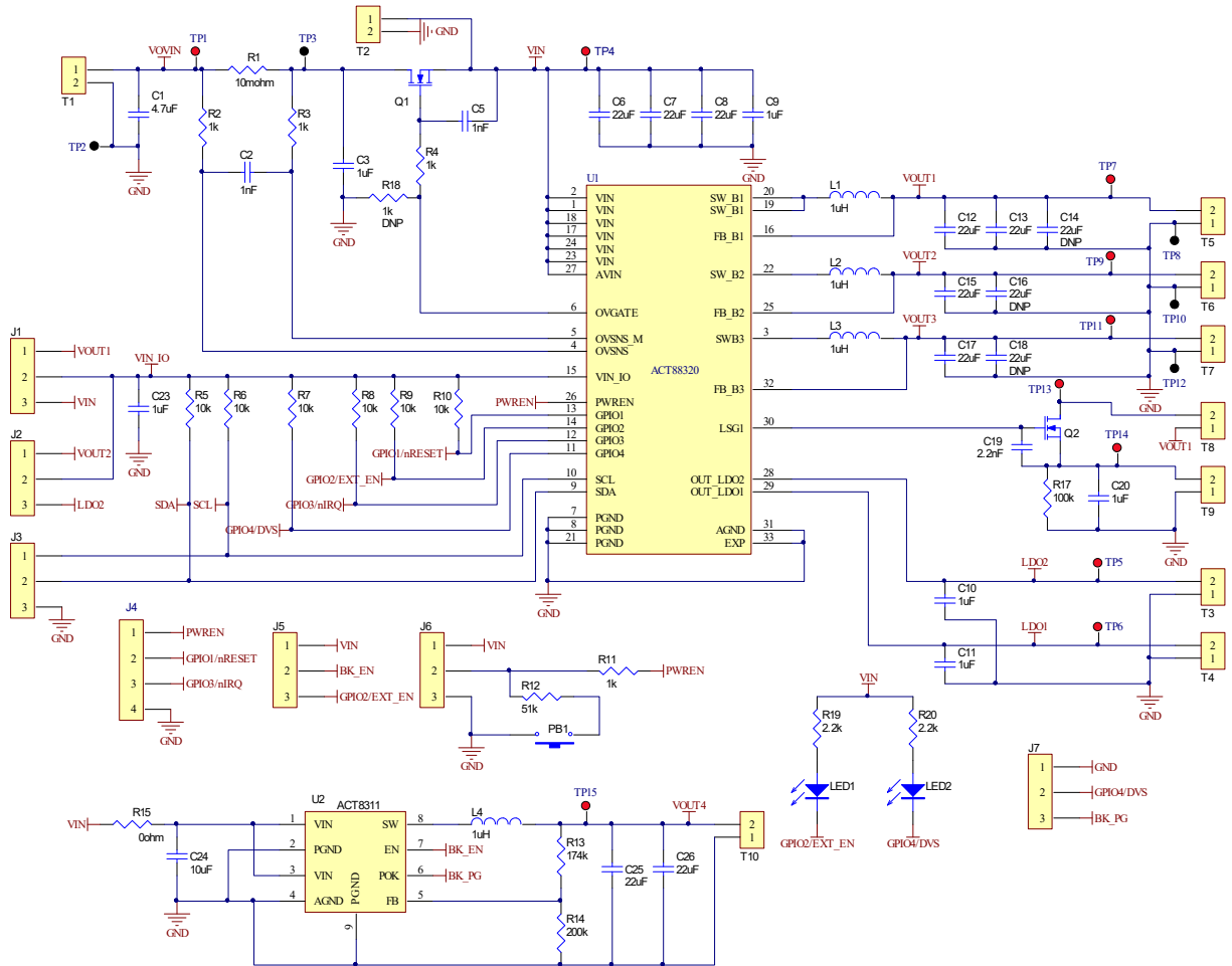
Figure 5 – ACT88320EVK1-101 Schematic
