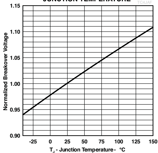
NORMALIZED BREAKOVER VOLTAGE vs JUNCTION TEMPERATURE
