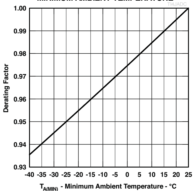
V_{DRM} DERATING FACTOR vs MINIMUM AMBIENT TEMPERATURE
