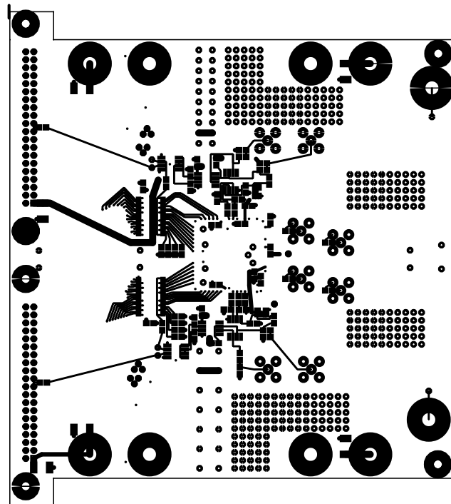
Figure 10a. Bottom View
