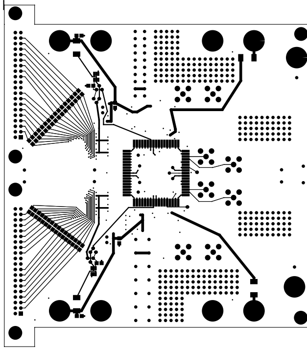
Figure 10e. Bottom Silk
