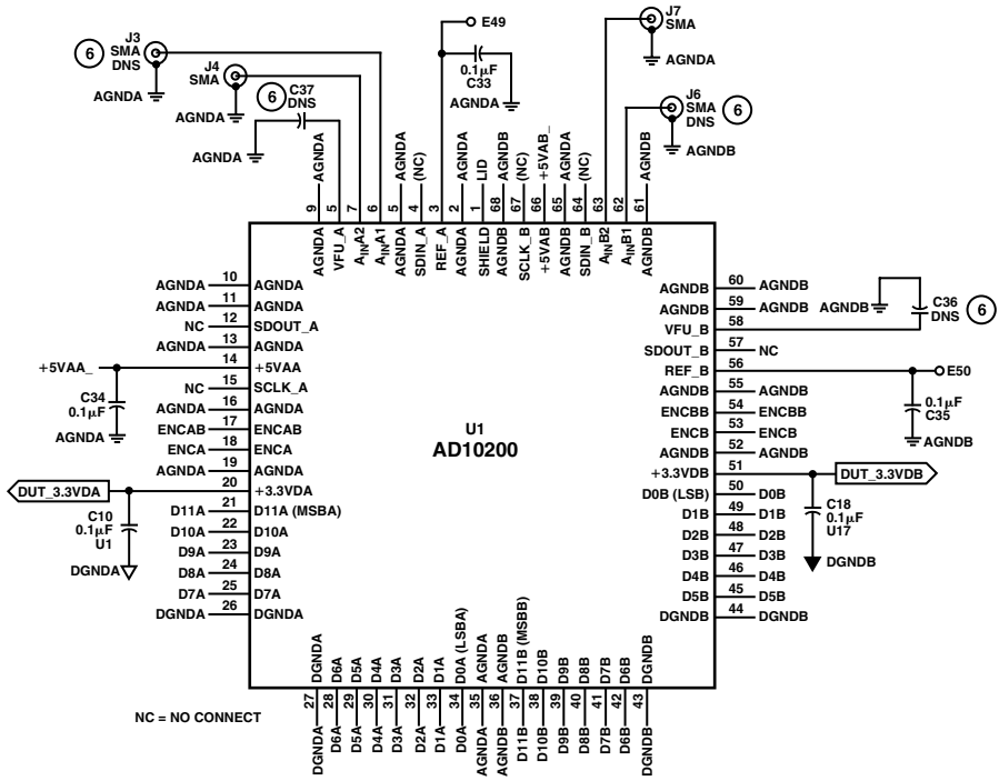
Figure 9a. Evaluation Board
