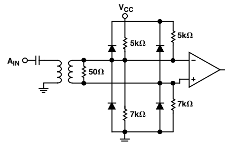
Figure 5. Equivalent Analog Input Circuit
