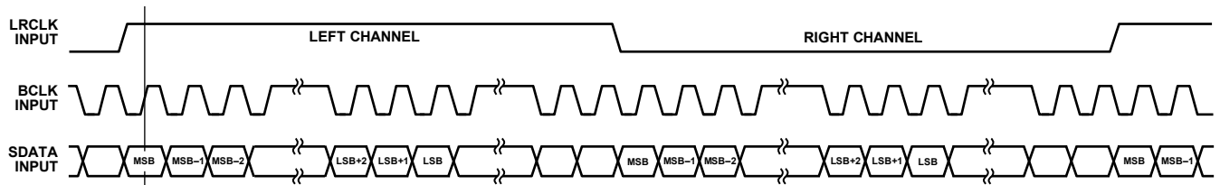
Figure 5. Left-Justified Mode
