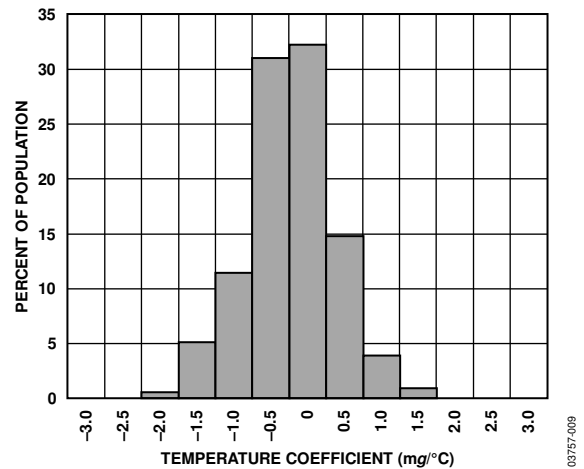
Figure 29. Y-Axis Zero g Bias Temperature Coefficient
