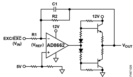
Figure 27. Buffer Circuit
