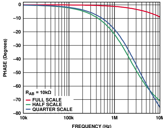
Figure 18. Normalized Phase Flatness vs. Frequency
