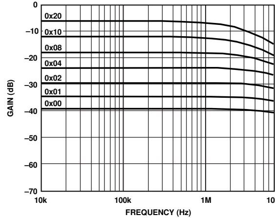
Figure 17. 10 kΩ Gain vs. Frequency vs. Code
