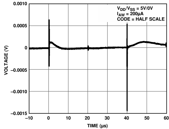
Figure 35. Digital Feedthrough
