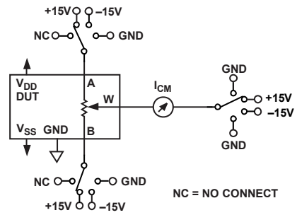
Figure 37. Common-Mode Leakage Current
