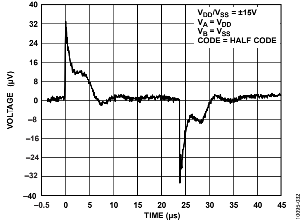
Figure 27. Digital Feedthrough
