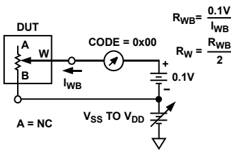
Figure 34. Wiper Resistance
