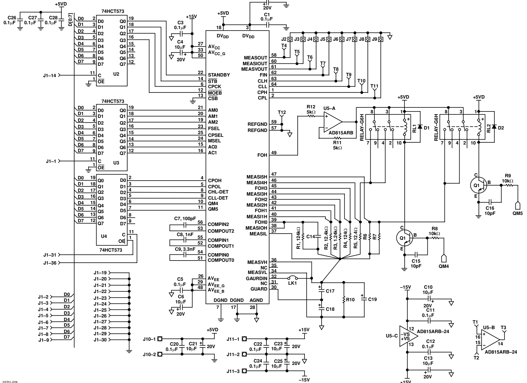
Figure 28. Evaluation Board Schematic
