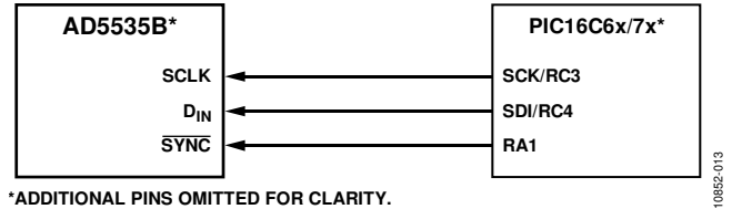
Figure 18. AD5535B-to-PIC16C6x/7x Interface
