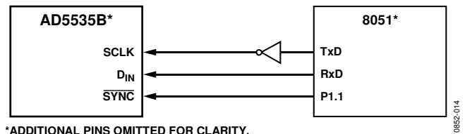
Figure 19. AD5535B-to-8051 Interface
