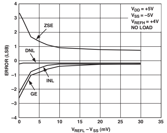
TPC 6. AD5582 INL, DNL, GE, and ZSE at Negative Rail-to-Rail Operation
