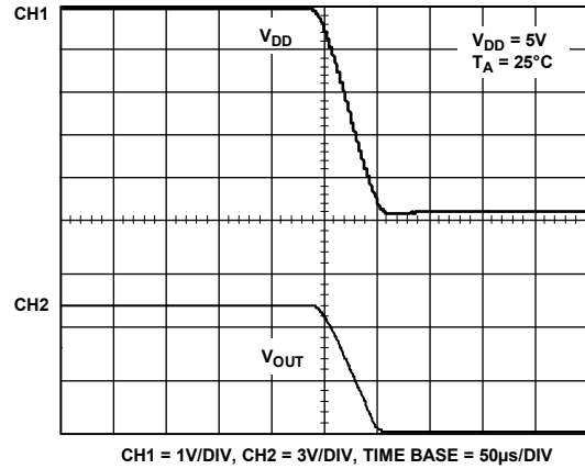
Figure 32. V_{OUT} vs. V_{DD}
