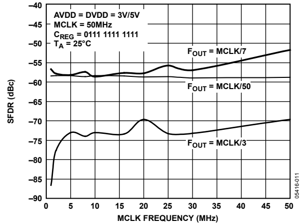
Figure 11. Wide-Band SFDR vs. MCLK Frequency
