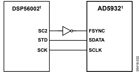
Figure 37. DSP56002 to AD5932 Interface
