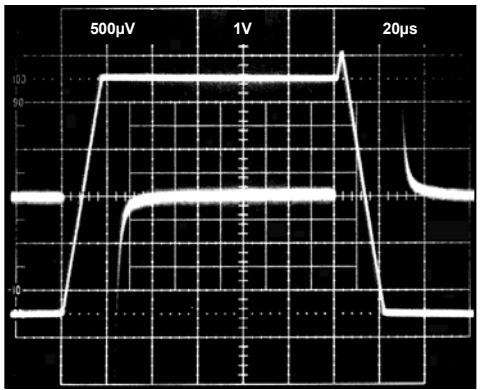
Figure 29. Large Signal Pulse Response and Settling Time, G = -1 ( 0.250 mV = 0.01%), C_L = 100 pF
