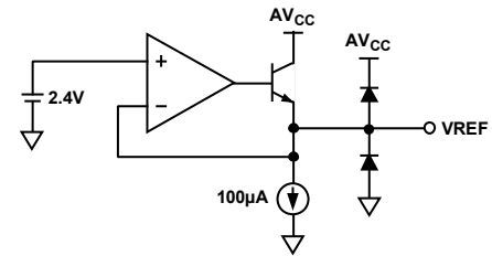
Figure 36. 2.4 V Reference
