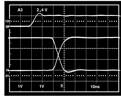
Figure 13. RS-422 Driver; R LDIFF = 100 Ω, C L1 = C L2 = 100 pF
