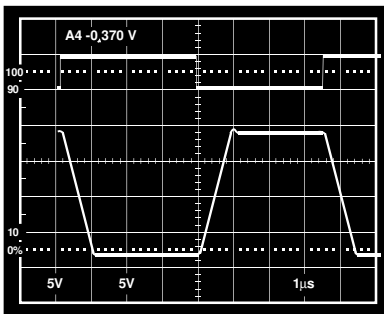
Figure 10. RS-232 Driver; R L = 5 kΩ, C L = 50 pF
