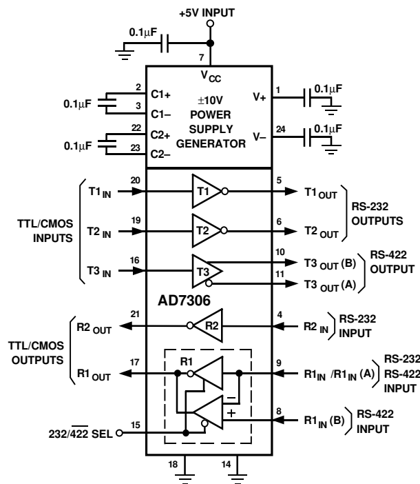
Figure 1. AD7306 Application Circuit
