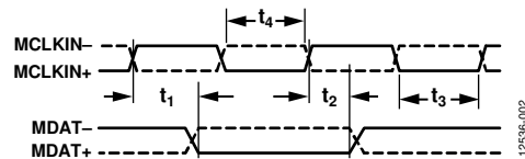
Figure 2. Data Timing
