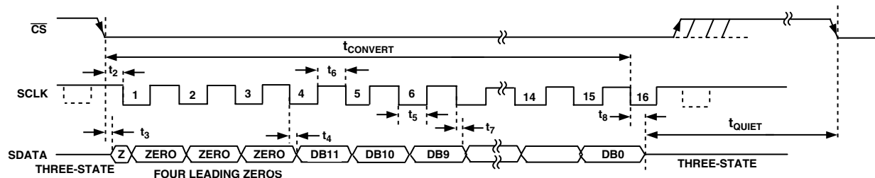
Figure 8. Serial Interface Timing Diagram Mode 1
