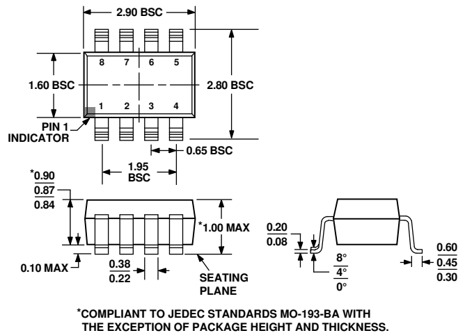
*COMPLIANT TO JEDEC STANDARDS MO-193-BA WITH THE EXCEPTION OF PACKAGE HEIGHT AND THICKNESS. Figure 36. 8-Lead Thin Small Outline Transistor Package [TSOT] (UJ-8) Dimensions shown in millimeters
