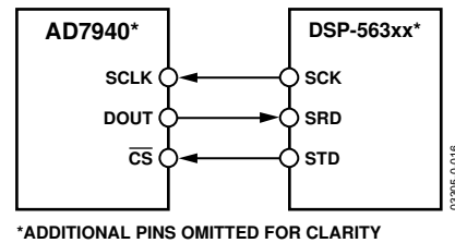
Figure 23. Interfacing to the DSP-563xx
