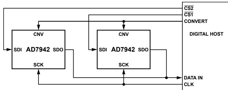
Figure 34. \overline{CS} Mode 4-Wire Without Busy Indicator Connection Diagram
