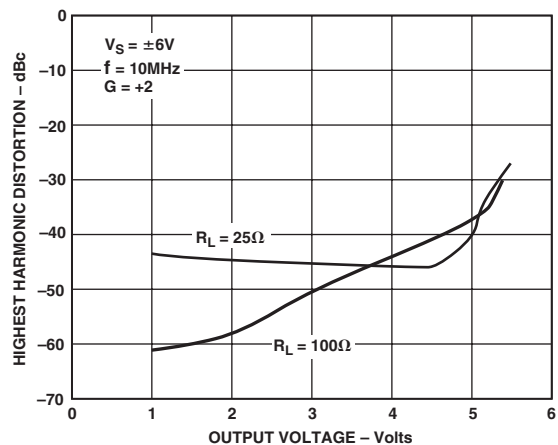
TPC 13. Distortion vs. Output Voltage, V_S = \pm 6\text{ V} , G = +2 , f = 10\text{ MHz}
