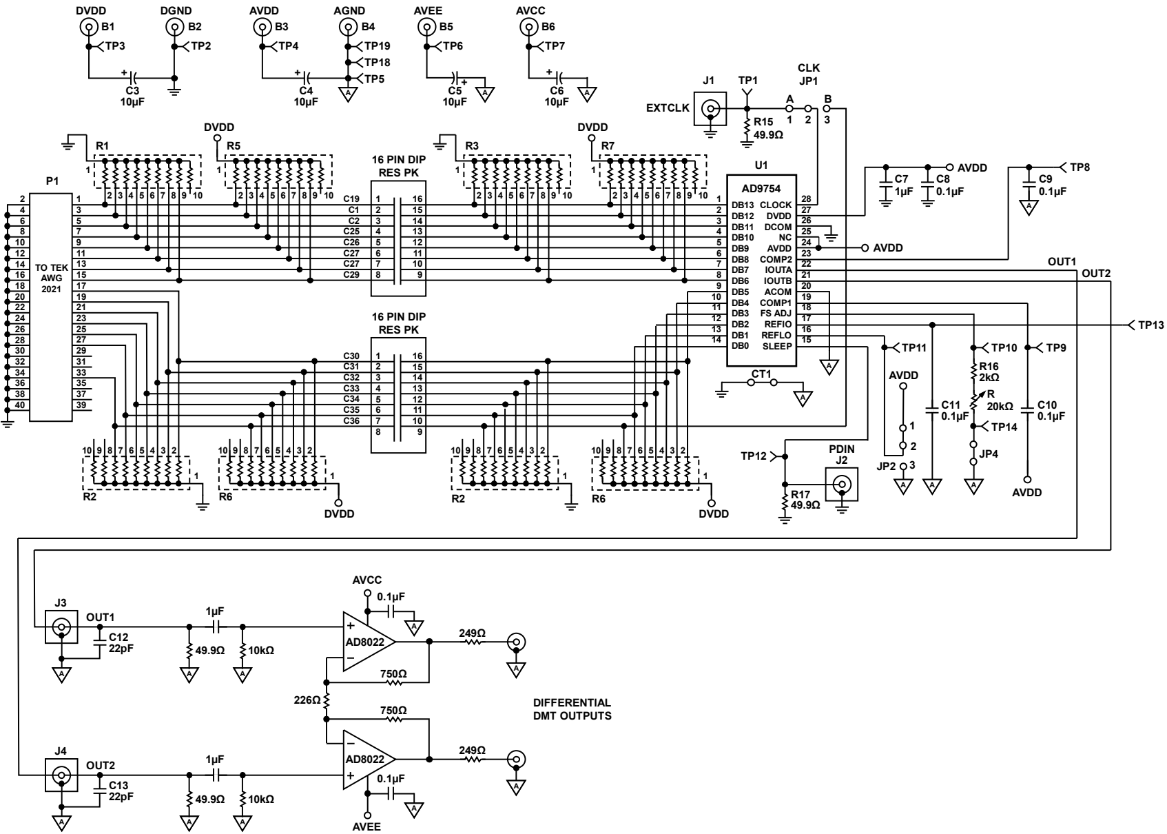
Figure 40. DMT Signal Generator Schematic
