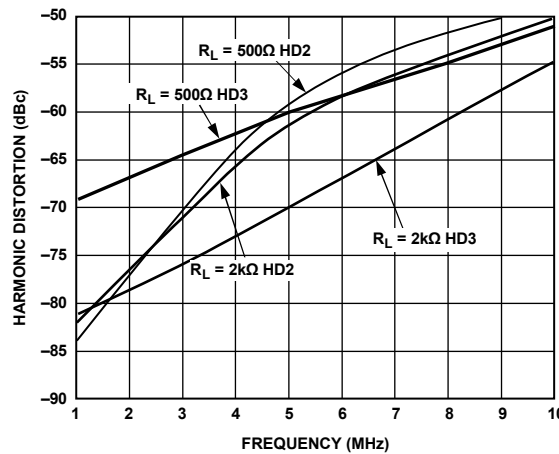
Figure 17. Harmonic Distortion vs. Frequency for Various Loads, V_S = \pm 5\text{ V} , V_{OUT} = 2\text{ V p-p} , G = +2
