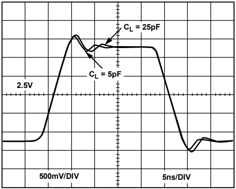
Figure 31. Large Signal Transient Response for Various C_L , V_S = 5V
