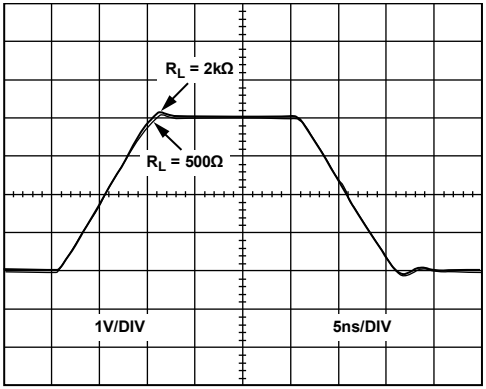
Figure 30. Large Signal Transient Response for Various R_L , V_S = \pm 5V
