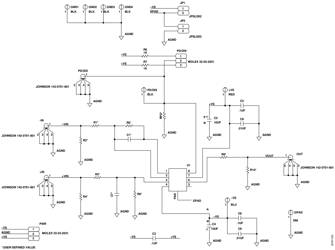
Figure 3. Evaluation Board Schematic
