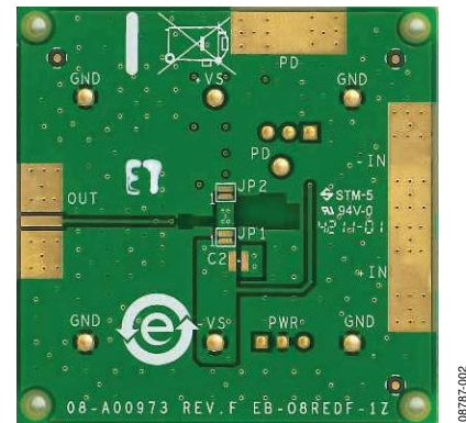
Figure 2. Circuit Side of the Evaluation Board
