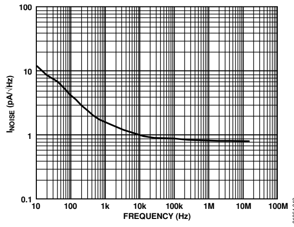
Figure 39. Current Noise vs. Frequency
