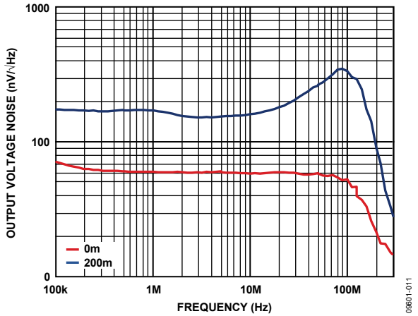
Figure 11. Output Voltage Noise vs. Frequency for Various Cable Lengths
