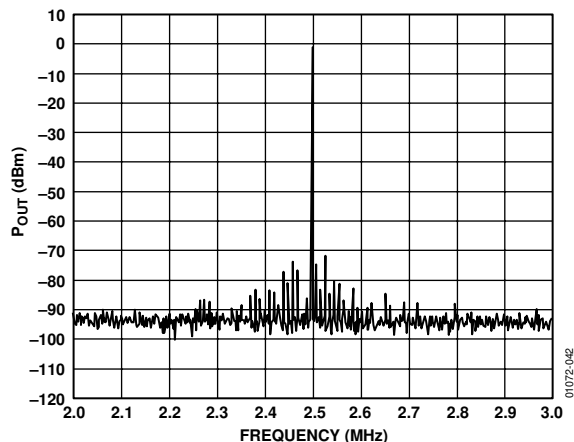
Figure 42. FFT Plot for AD8131/AD9203
