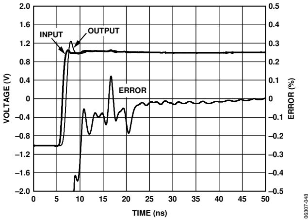
Figure 22. Settling Time
