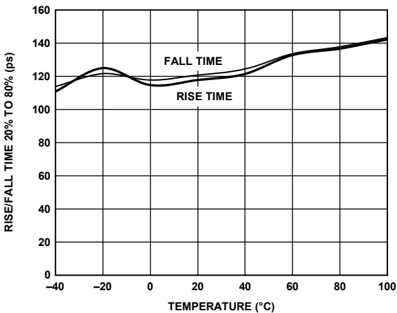
Figure 22. Rise/Fall Time vs. Temperature
