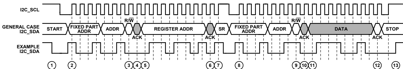
Figure 30. I 2 C Read Diagram
