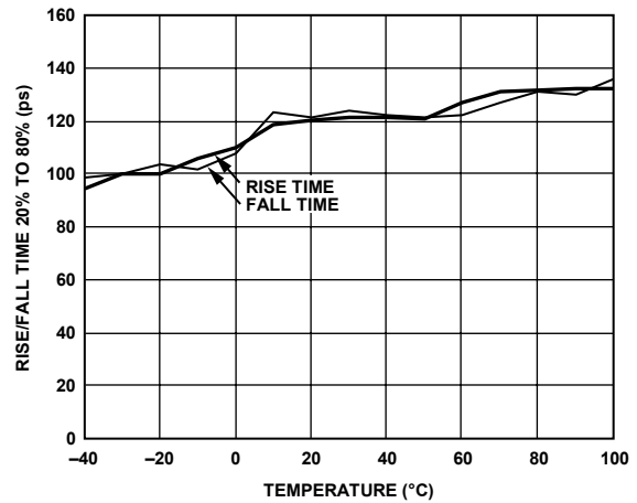
Figure 18. Rise and Fall Time vs. Temperature
