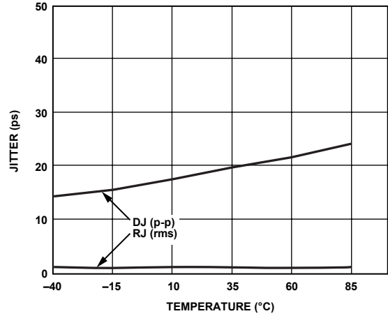
Figure 17. Jitter vs. Temperature
