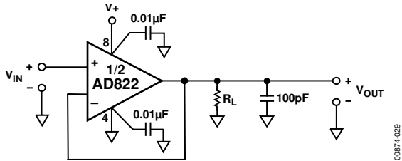
Figure 29. Unity-Gain Follower
