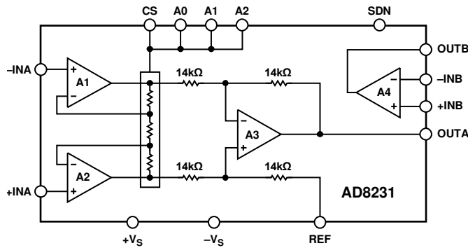
Figure 49. Simplified Schematic
