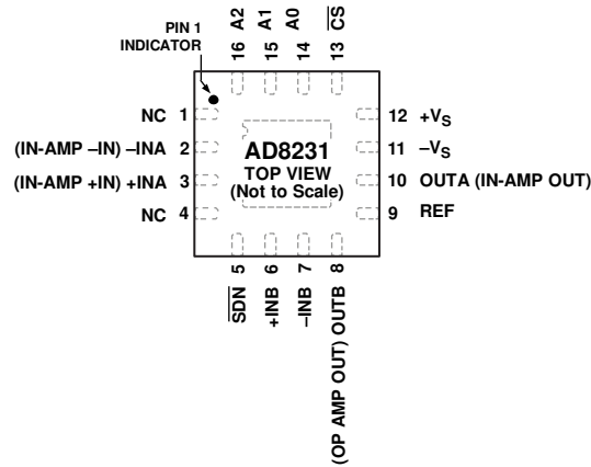
Figure 2. Pin Configuration
