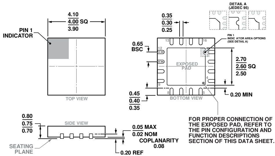
Figure 57. 16-Lead Lead Frame Chip Scale Package [LFCSP] 4 mm × 4 mm Body and 0.75mm Package Height (CP-16-17) Dimensions shown in millimeters
