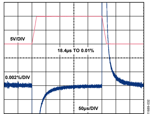
Figure 32. Large Signal Pulse Response and Settling Time, R_L = 10\text{ k}\Omega , C_L = 100\text{ pF}
