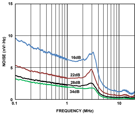
Figure 12. Short Circuit Input-Referred Noise vs. Frequency
