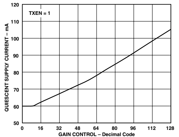
TPC 18. Supply Current vs. Gain Code
