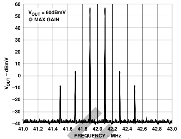
TPC 16. Two-Tone Intermodulation Distortion
