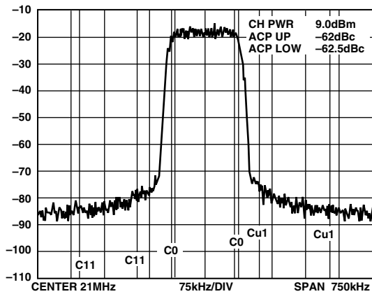
TPC 13. Adjacent Channel Power
