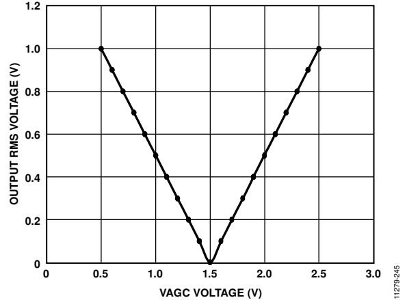
Figure 45. Output RMS Voltage vs. VAGC
