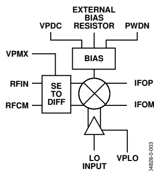
Figure 35. AD8344 Simplified Schematic
