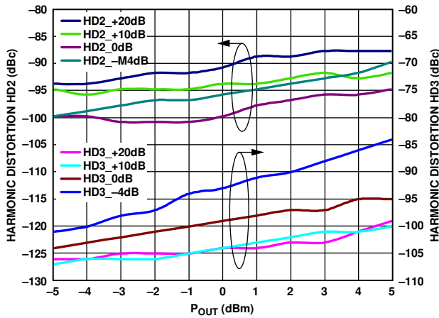
Figure 17. Harmonic Distortion vs. Power at Four Gain Codes, Frequency 140 MHz
