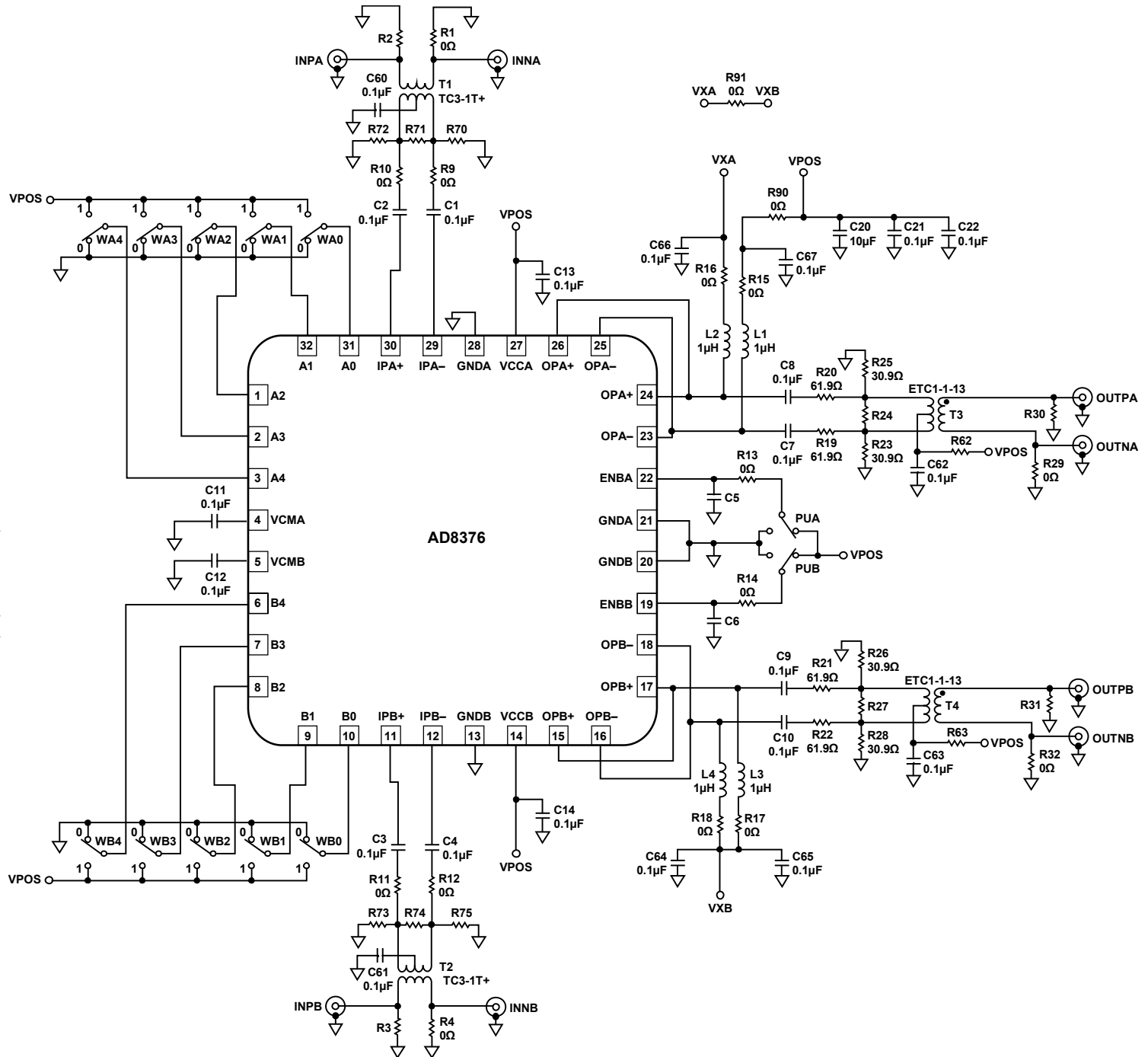
Figure 47. AD8376 Evaluation Board Schematic
