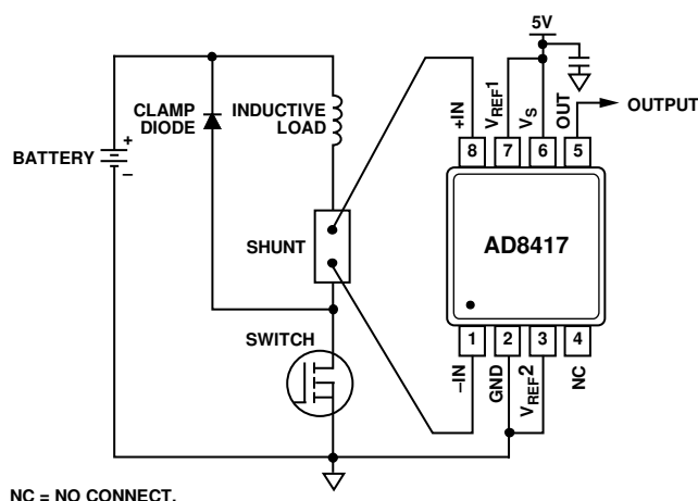
Figure 34. Low-Side Switch
