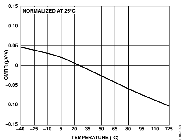
Figure 24. CMRR vs. Temperature
