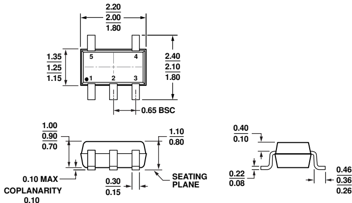
Figure 40. 5-Lead Small Outline Transistor Package [SOT-23] (RJ-5)
