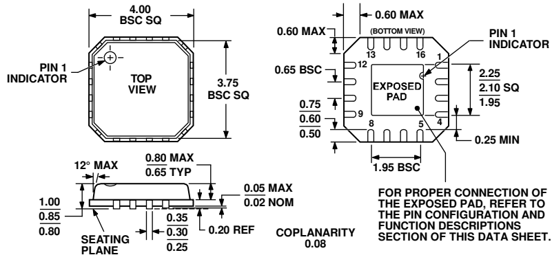
Figure 37. 16-Lead Lead Frame Chip Scale Package [LFCSP_VQ] 4 mm x 4 mm Body, Very Thin Quad (CP-16-4) Dimensions shown in millimeters
