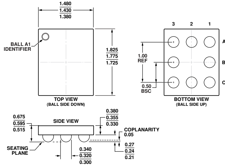
Figure 62. 8-Ball Wafer Level Chip Scale Package [WLCSPP] (CB-8-1) Dimensions shown in millimeters
