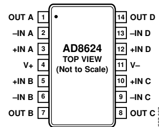
Figure 3. 14-Lead TSSOP
