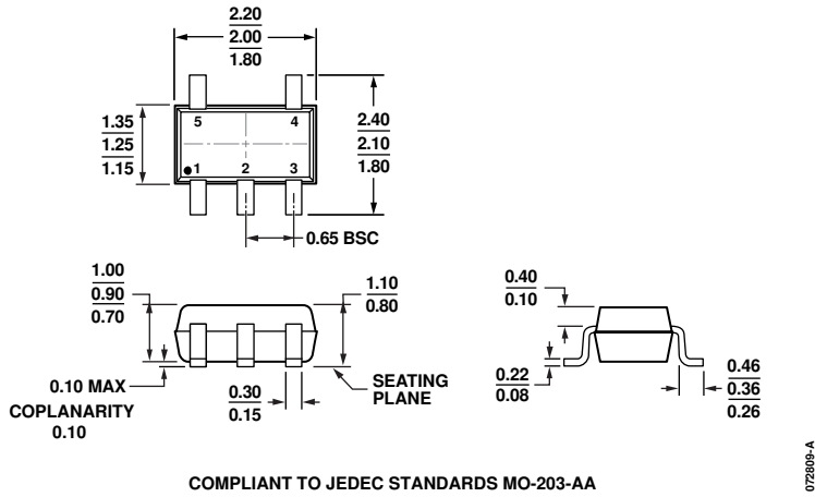
Figure 50. 5-Lead Plastic Surface-Mount Package [SC70] (KS-5) Dimensions shown in millimeters
