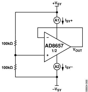
Figure 72. Voltage Follower
