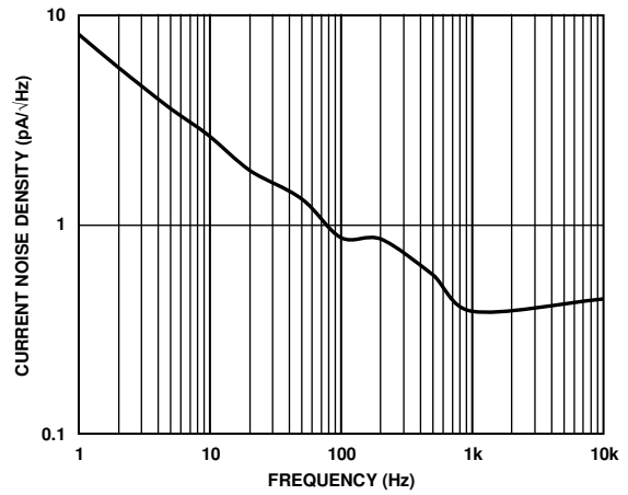
Figure 7. Current Noise Density V_S = \pm 15\text{ V}
