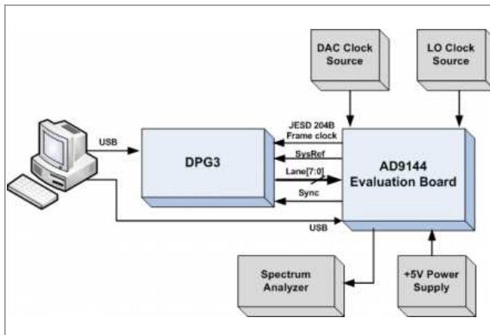
Figure 1. Block diagram of the AD9144 lab bench set-up
