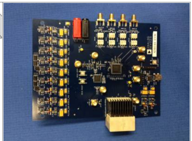
Figure 2. Top view of AD9144-EBZ
